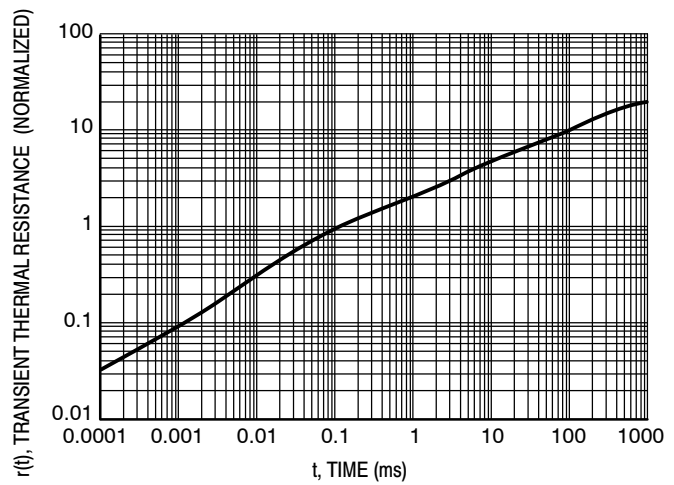
Figure 4. Thermal Response
