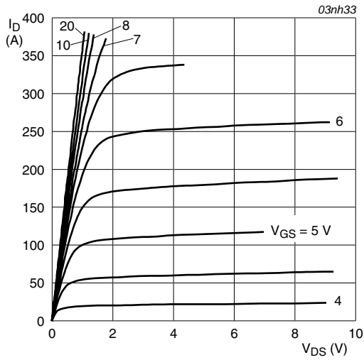
T_j = 25^\circ C; t_p = 300\mu s
