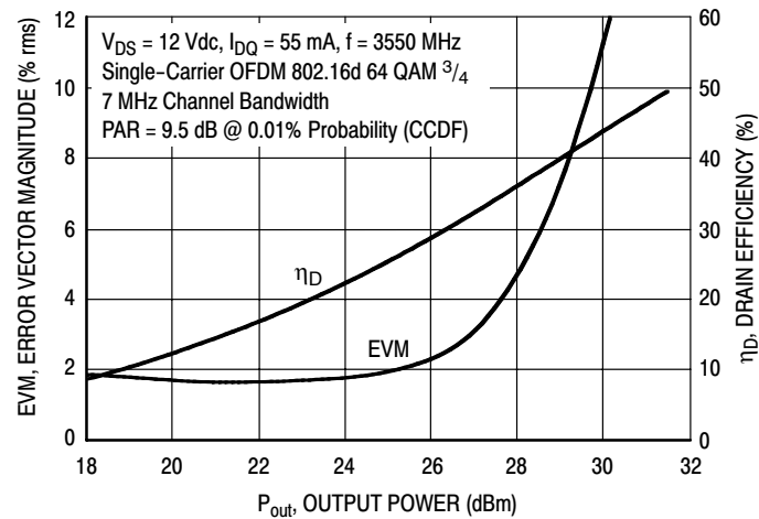
Figure 9. Single-Carrier OFDM EVM and Drain Efficiency versus Output Power
