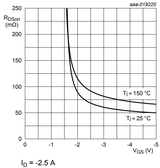
Fig. 10. Drain-source on-state resistance as a function of gate-source voltage; typical values I_D = -2.5\text{ A}
