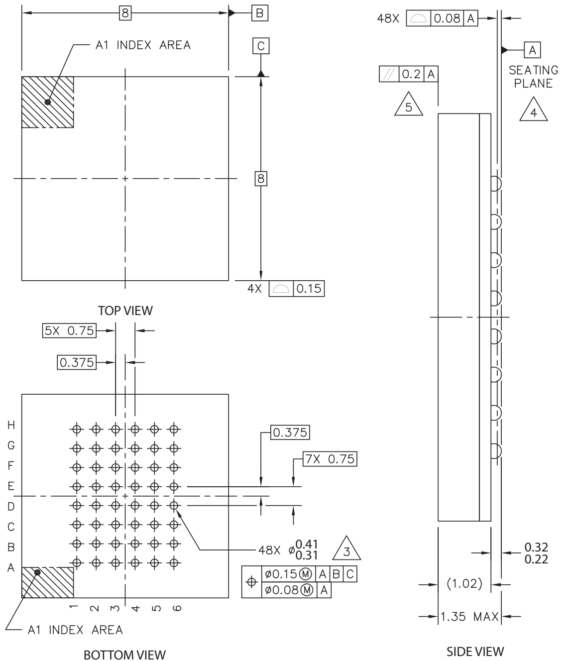
Figure 5.1 FBGA
