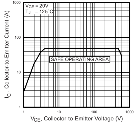
Fig. 12 - Turn-Off SOA
