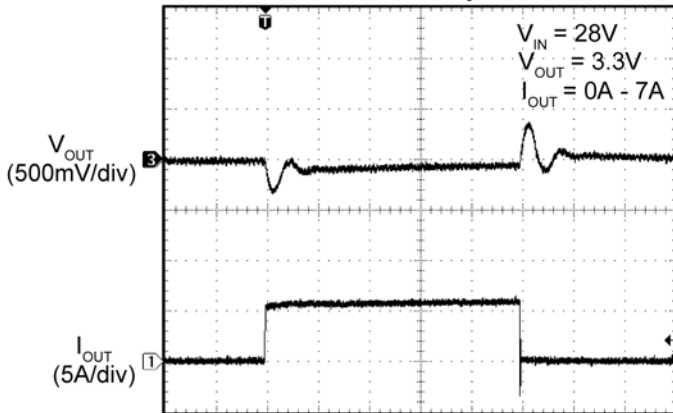
Transient Response
