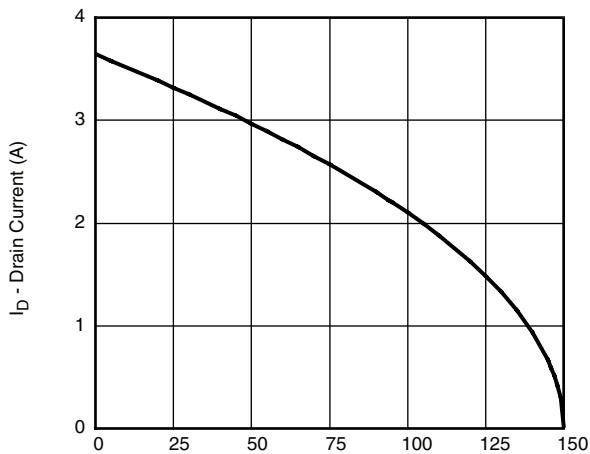
T_C - Case Temperature ( ^\circ\text{C} ) Current Derating*
